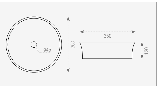
188621 Lavabo Terrazo 35x35x12 cm./13.8"x13.8"x4.7" E800
